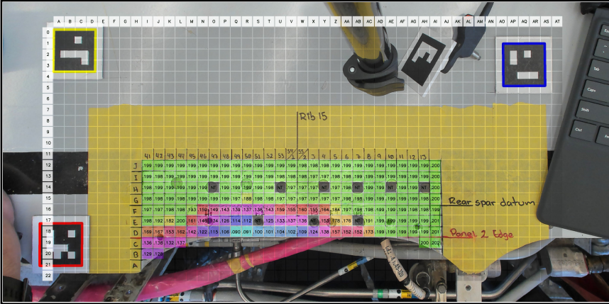
C-Scan Mosaic
